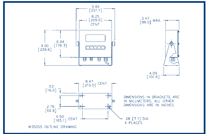
350 STAINLESS STEEL ENCLOSURE
